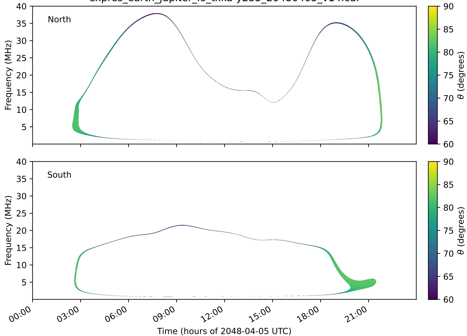
expres_earth_jupiter_io_txka-y235_20480405_v14.cdf
