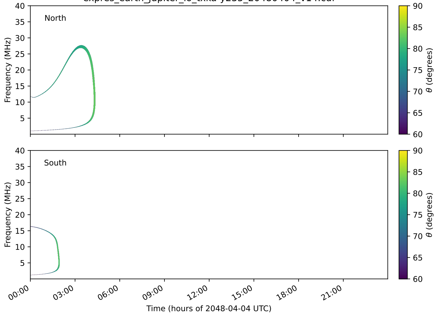
expres_earth_jupiter_io_txka-y235_20480404_v14.cdf
