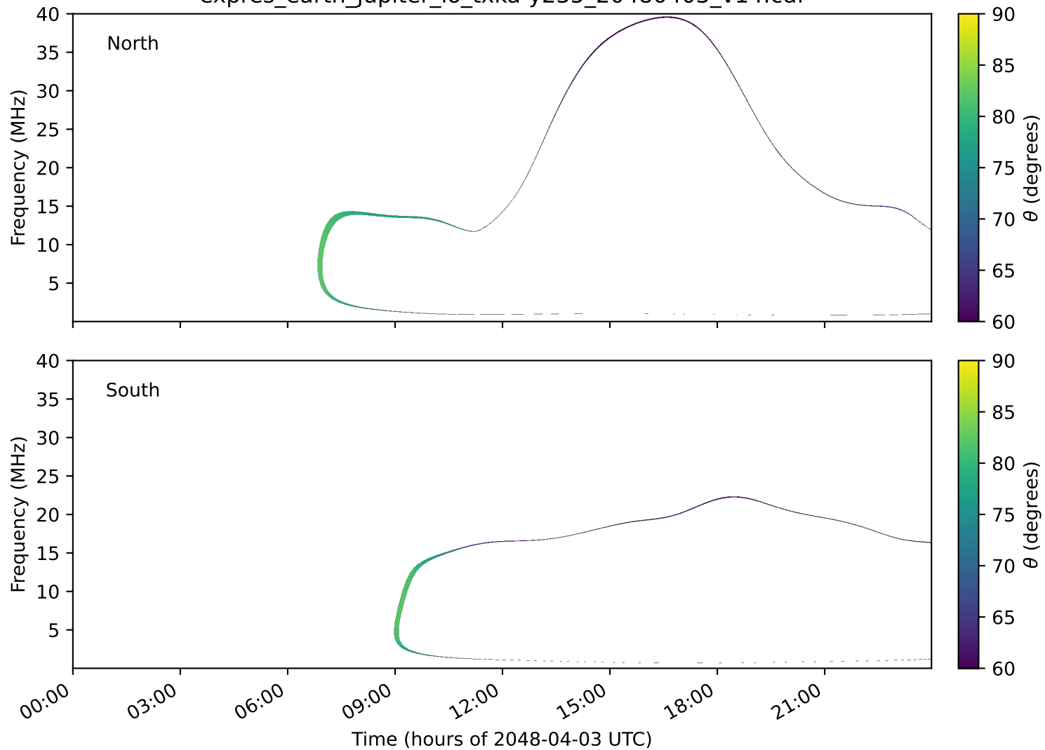
expres_earth_jupiter_io_txka-y235_20480403_v14.cdf
