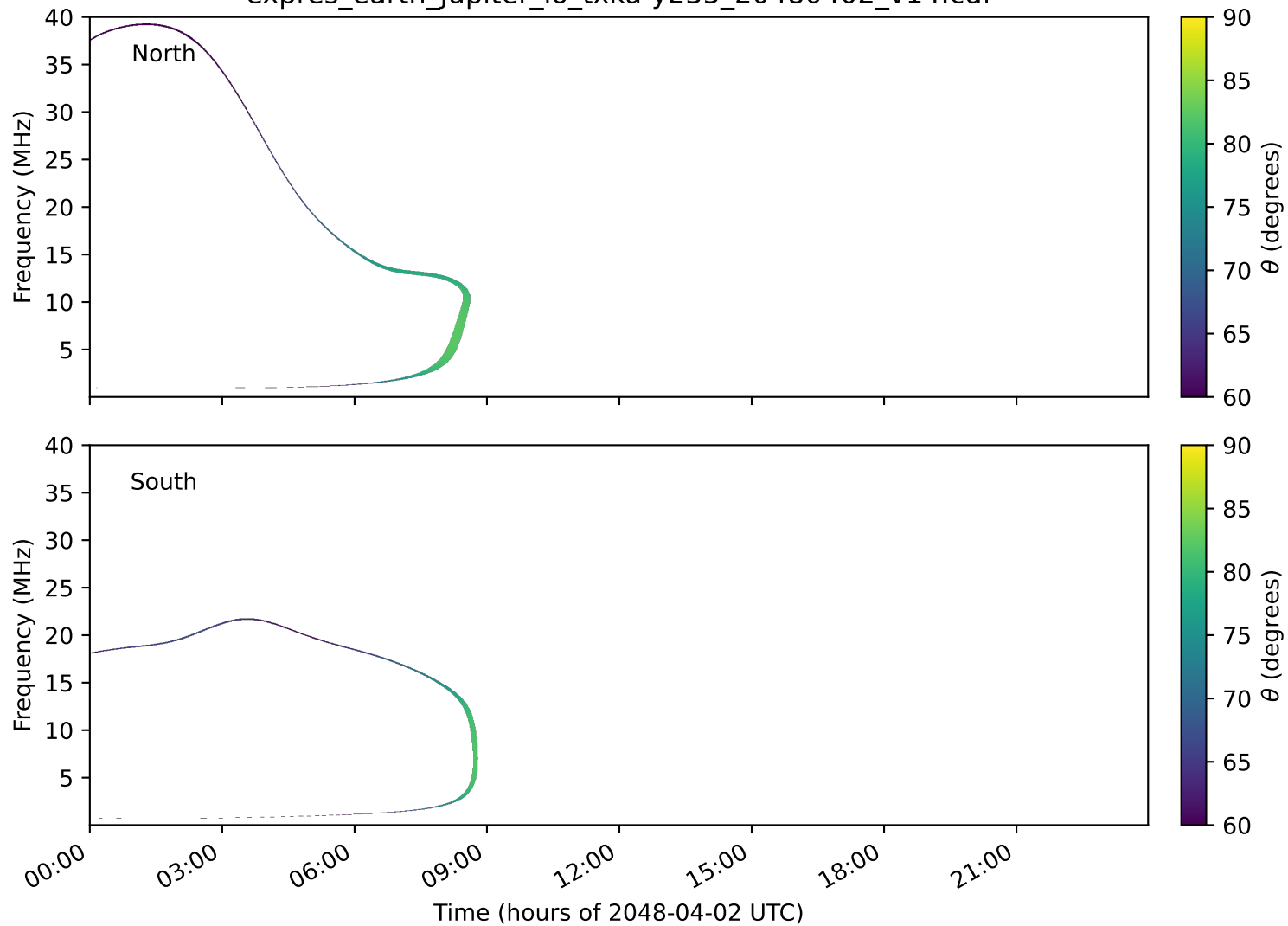
expres_earth_jupiter_io_txka-y235_20480402_v14.cdf
