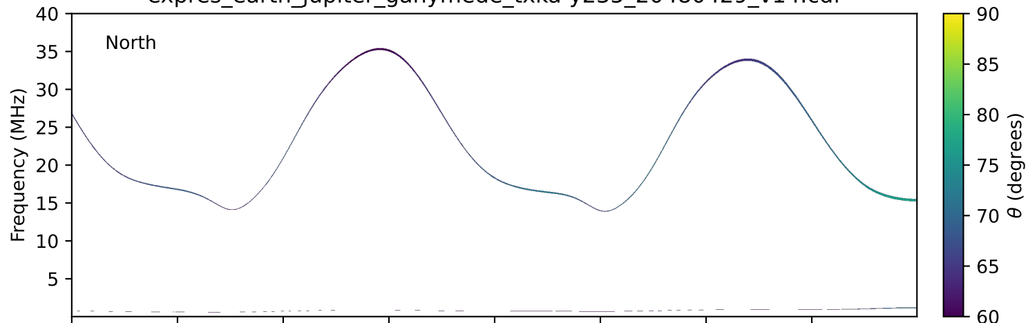
expres_earth_jupiter_ganymede_txka-y235_20480429_v14.cdf
