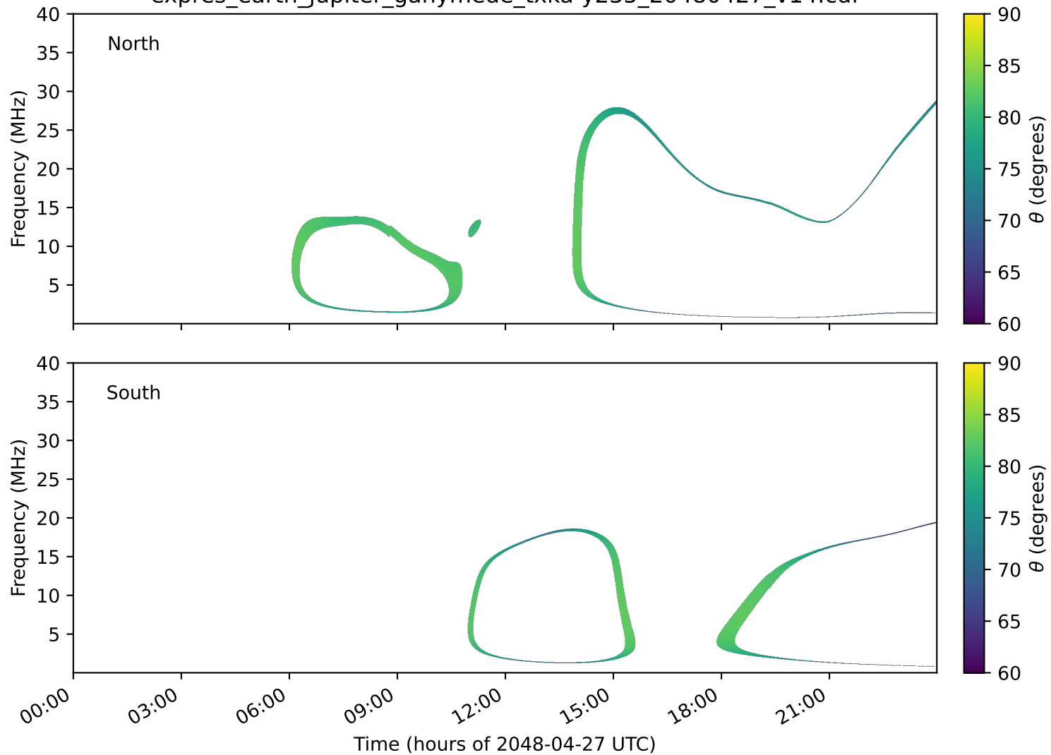
expres_earth_jupiter_ganymede_txka-y235_20480427_v14.cdf
