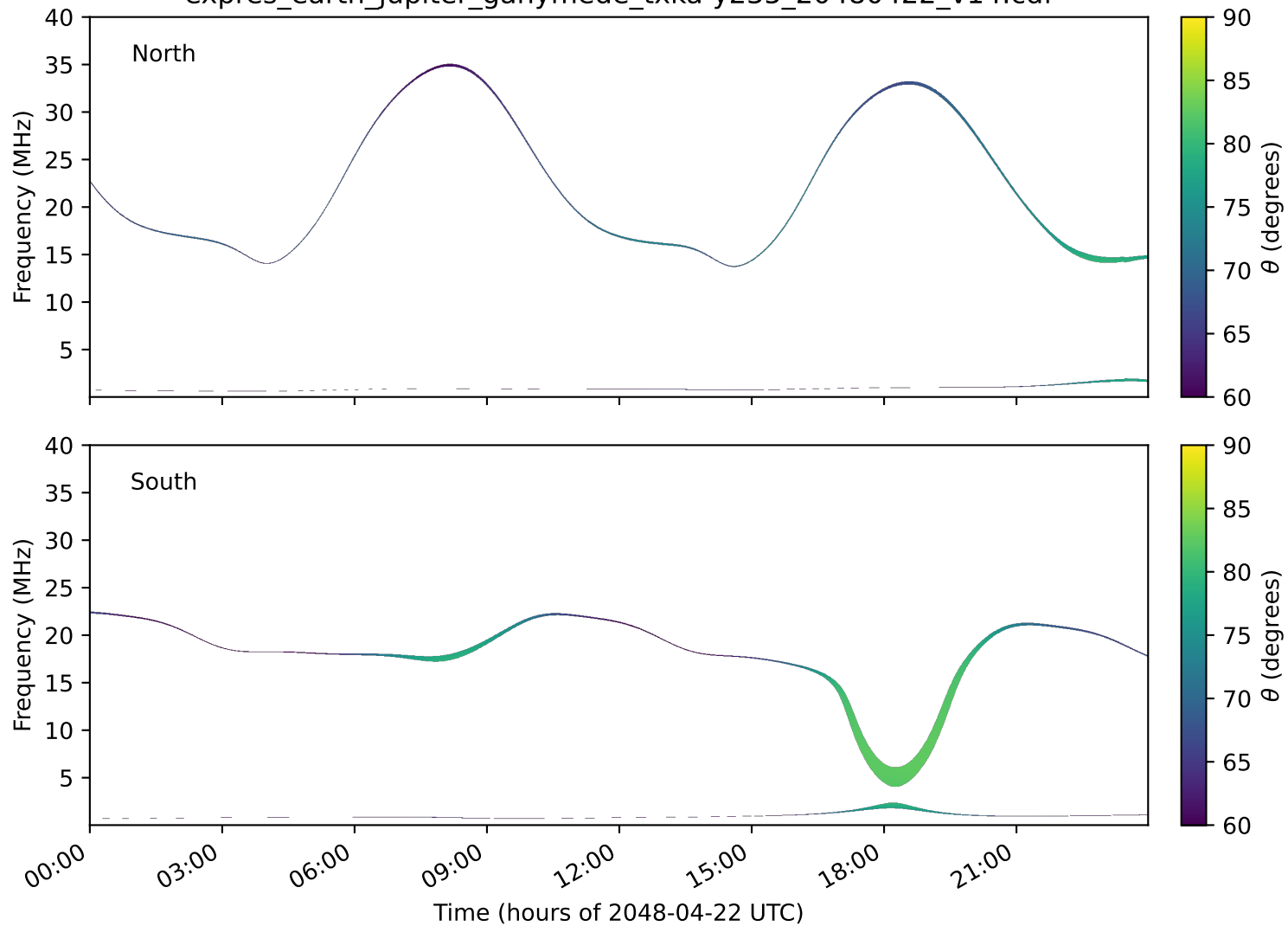
expres_earth_jupiter_ganymede_txka-y235_20480422_v14.cdf
