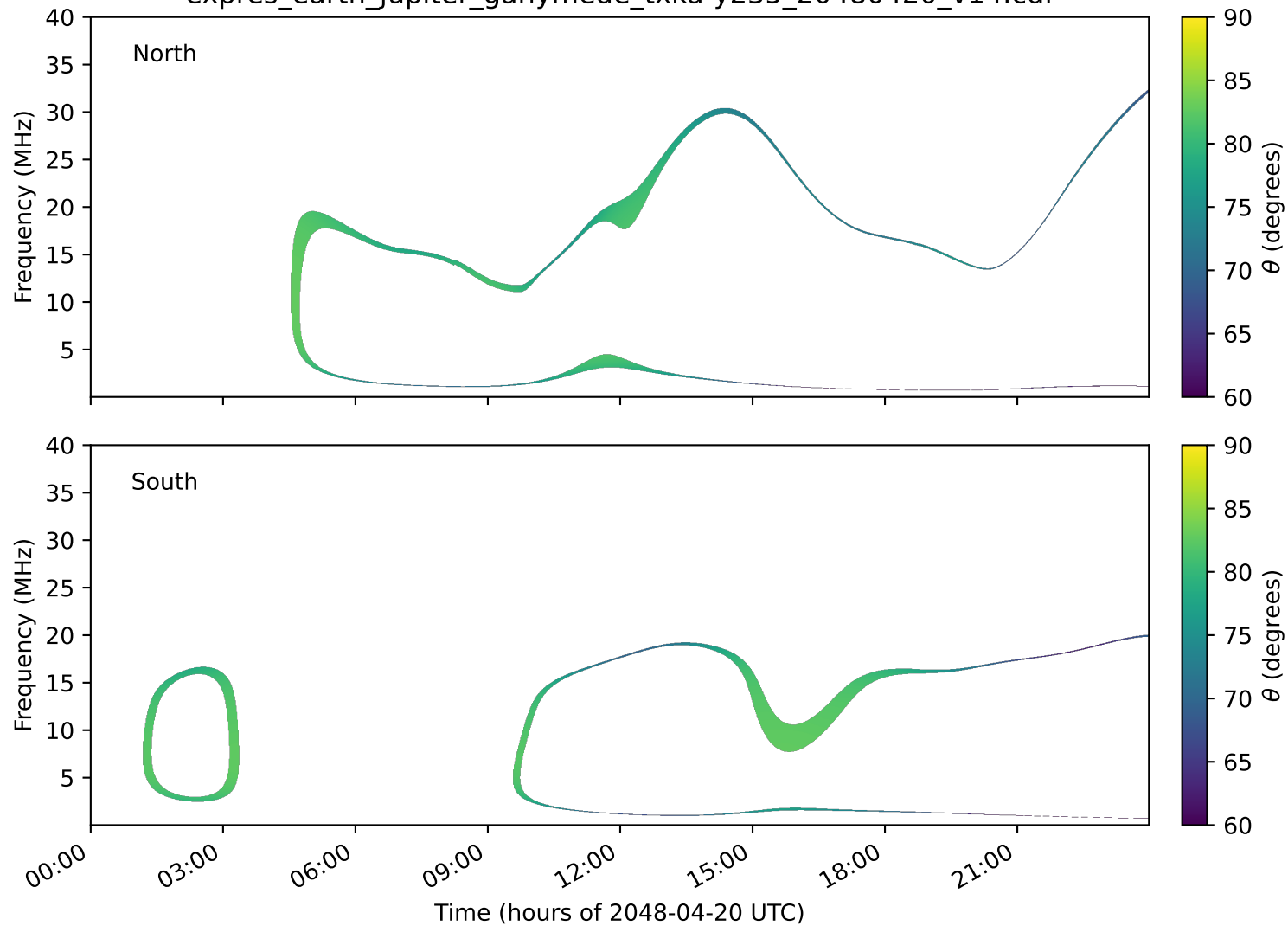
expres_earth_jupiter_ganymede_txka-y235_20480420_v14.cdf
