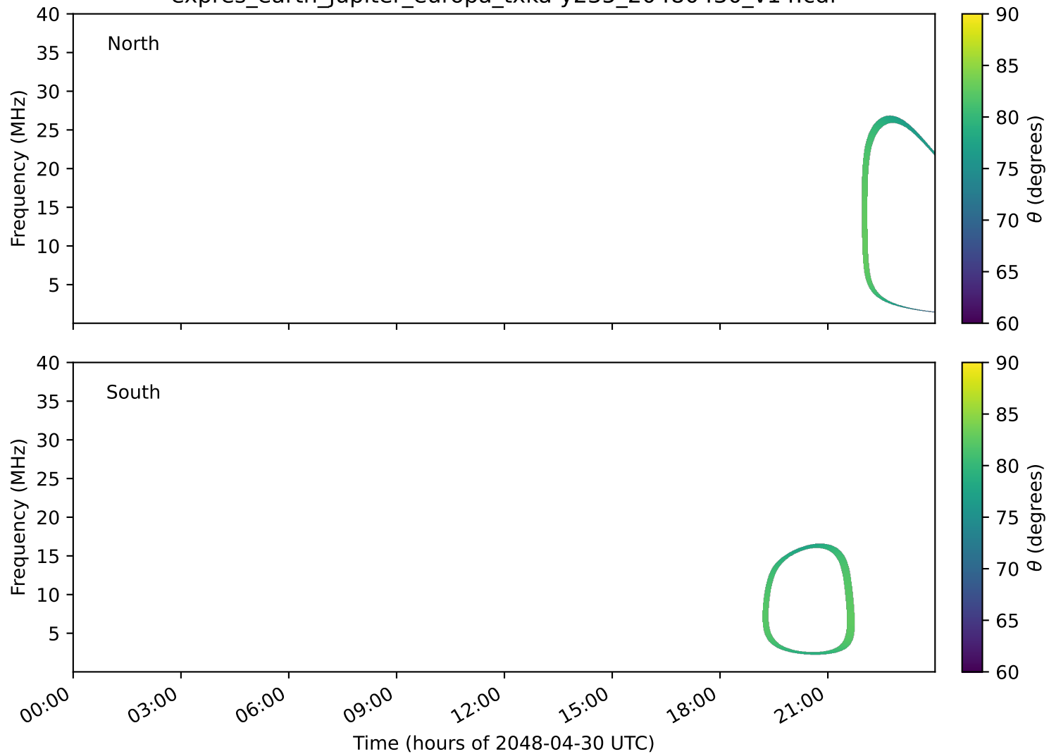
expres_earth_jupiter_europa_txka-y235_20480430_v14.cdf
