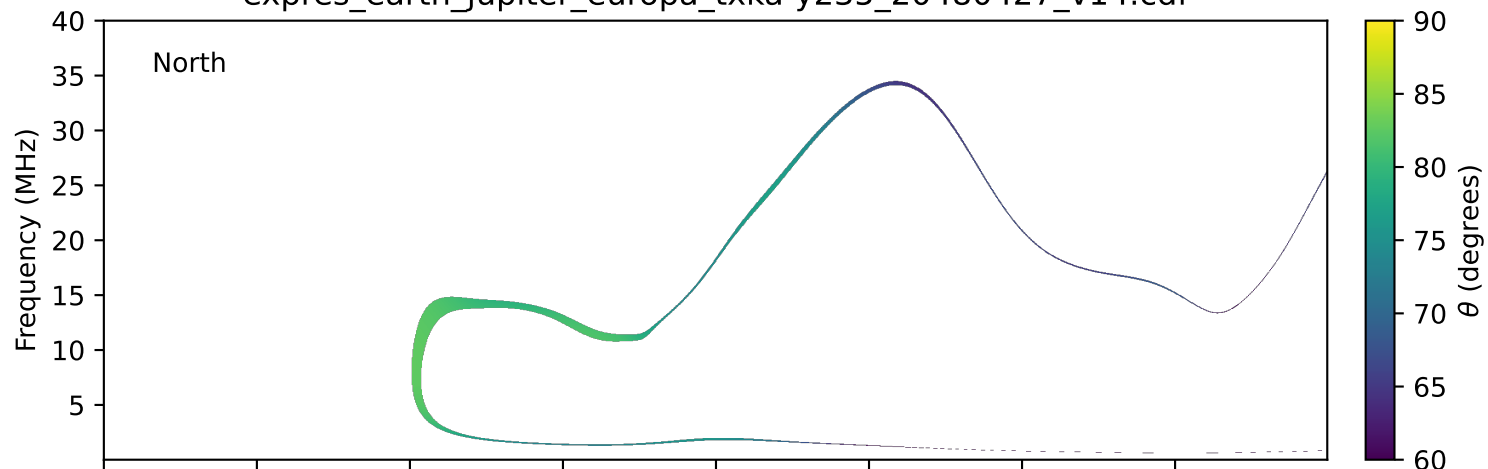
expres_earth_jupiter_europa_txka-y235_20480427_v14.cdf
