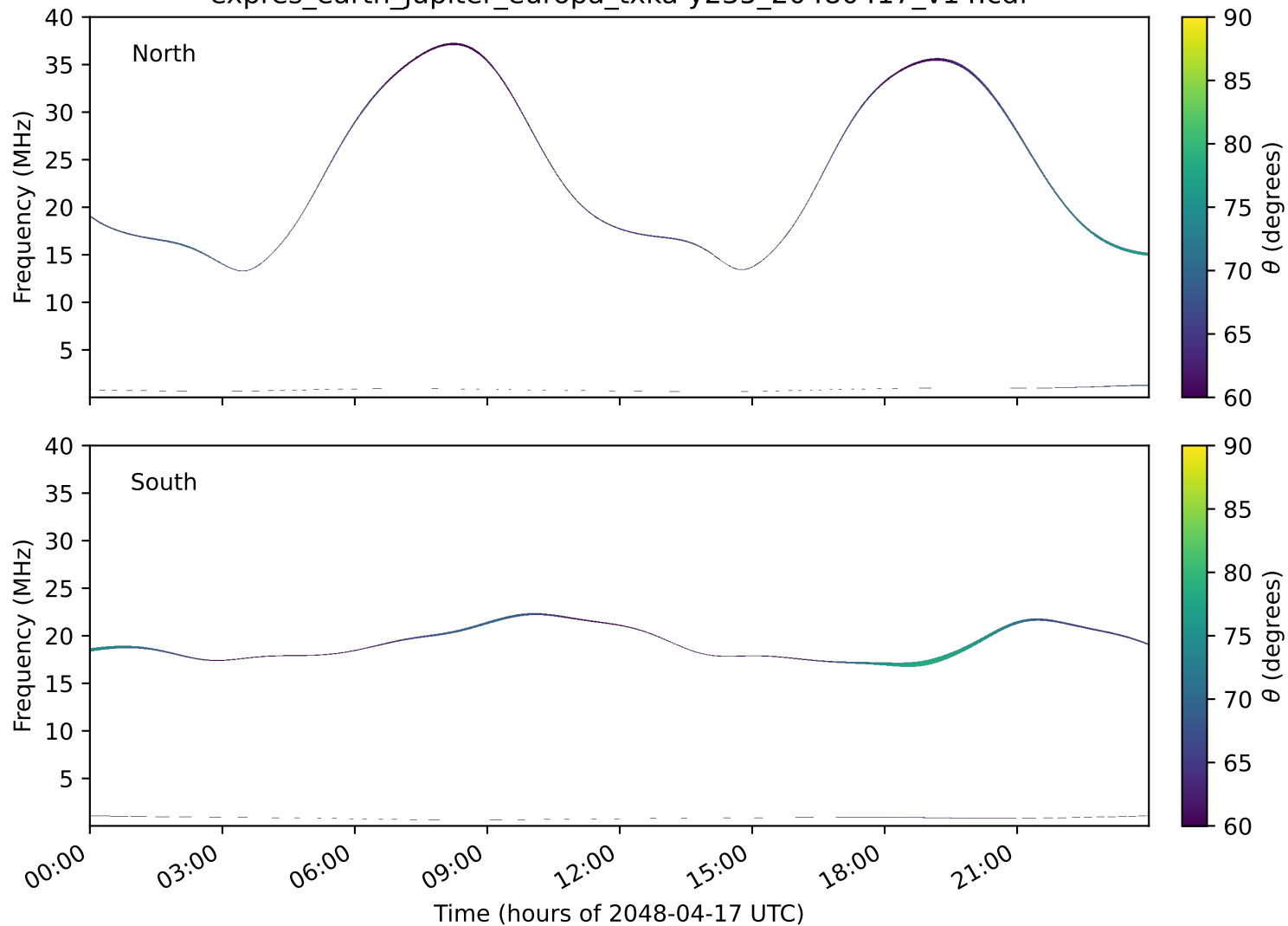
expres_earth_jupiter_europa_txka-y235_20480417_v14.cdf
