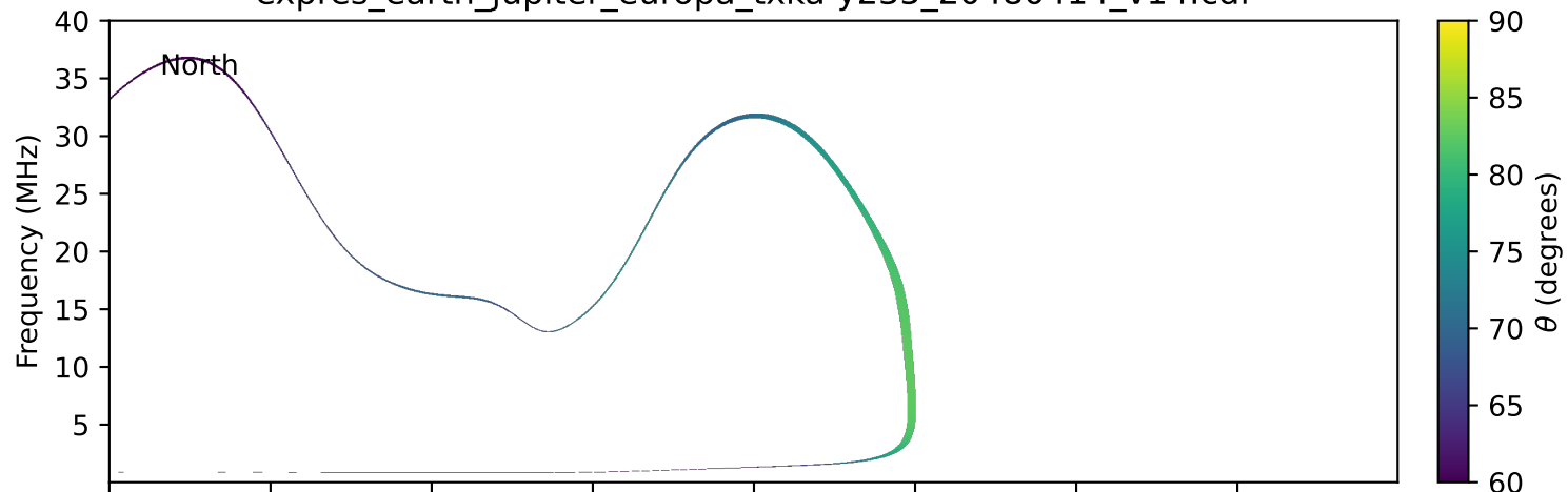
expres_earth_jupiter_europa_txka-y235_20480414_v14.cdf
