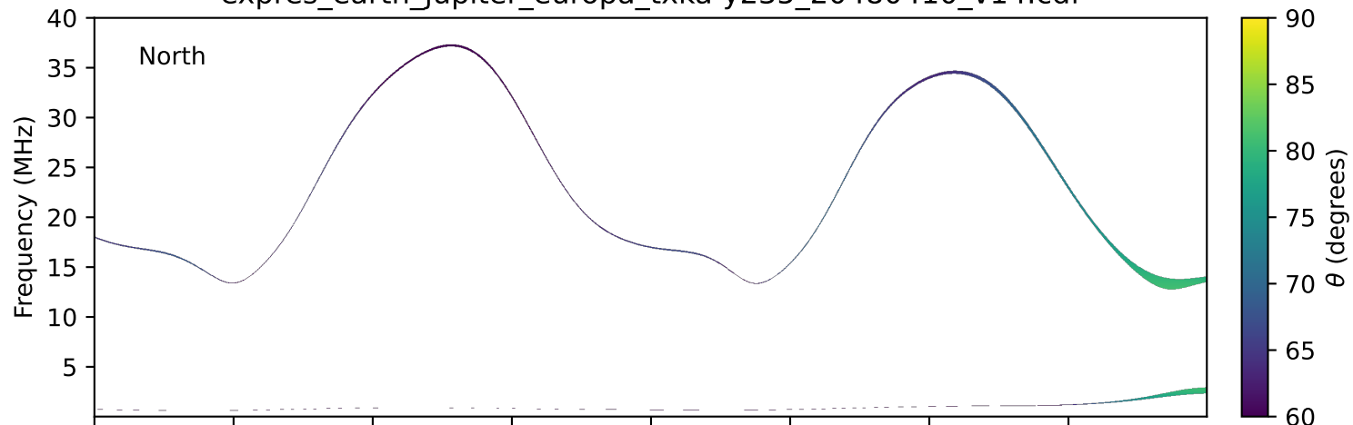
expres_earth_jupiter_europa_txka-y235_20480410_v14.cdf
