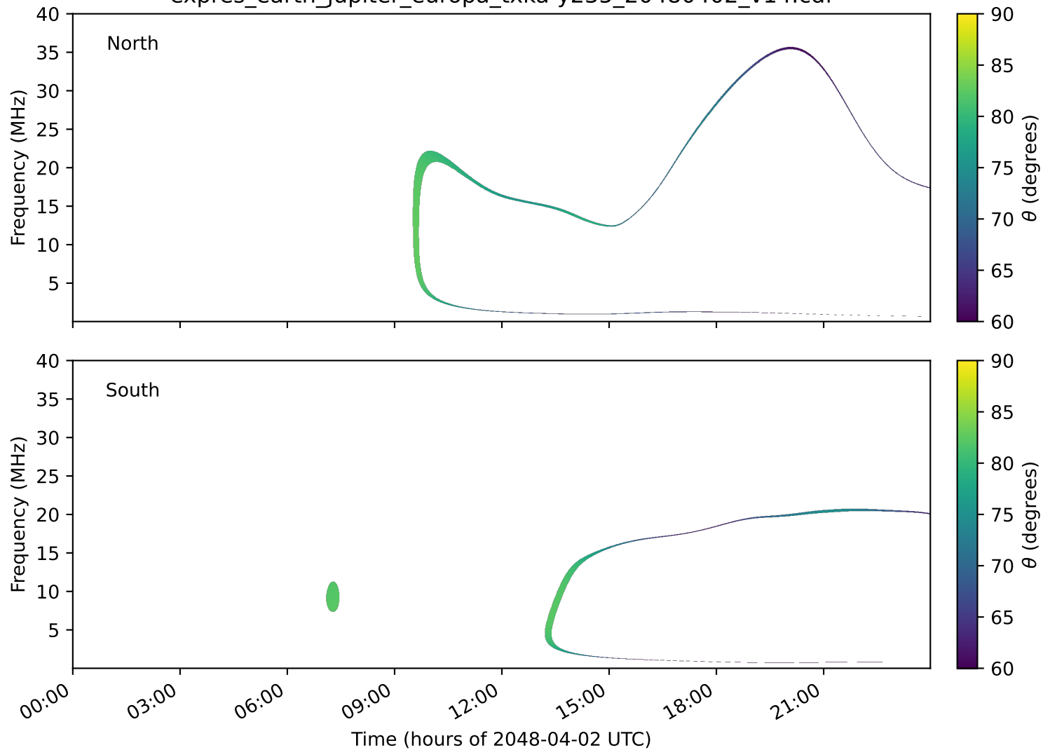
expres_earth_jupiter_europa_txka-y235_20480402_v14.cdf
