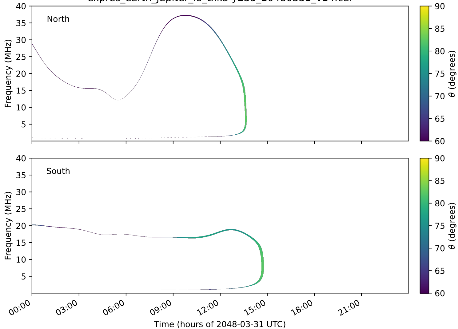
expres_earth_jupiter_io_txka-y235_20480331_v14.cdf
