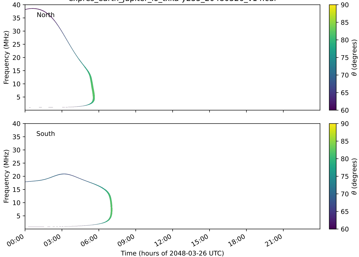
expres_earth_jupiter_io_txka-y235_20480326_v14.cdf
