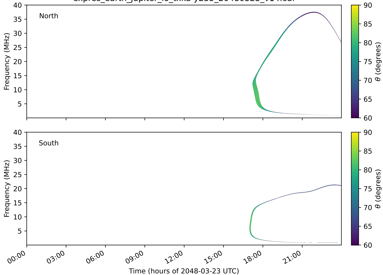
expres_earth_jupiter_io_txka-y235_20480323_v14.cdf
