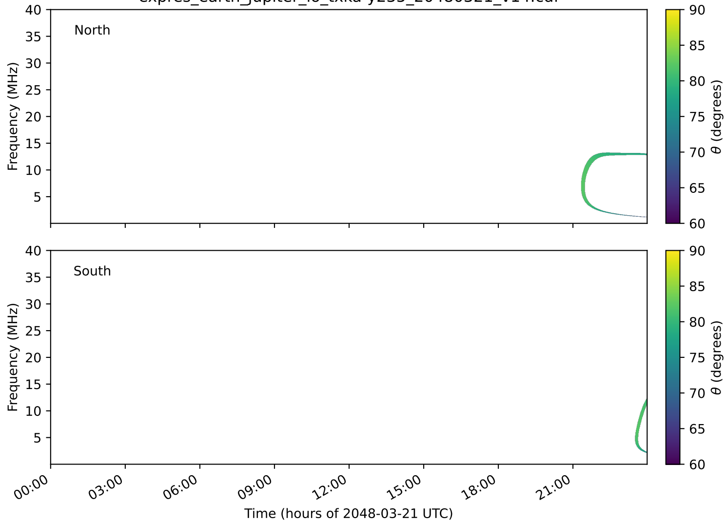
expres_earth_jupiter_io_txka-y235_20480321_v14.cdf
