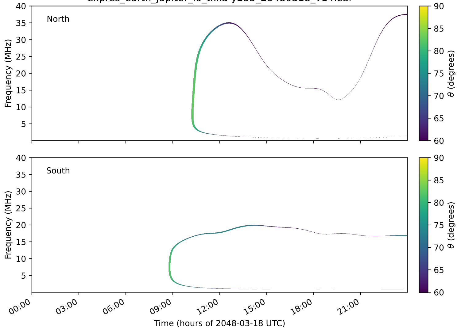
expres_earth_jupiter_io_txka-y235_20480318_v14.cdf
