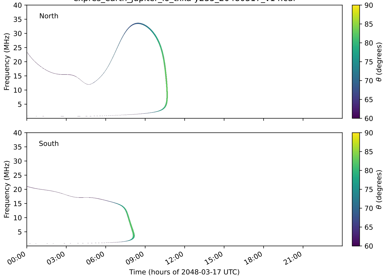
expres_earth_jupiter_io_txka-y235_20480317_v14.cdf
