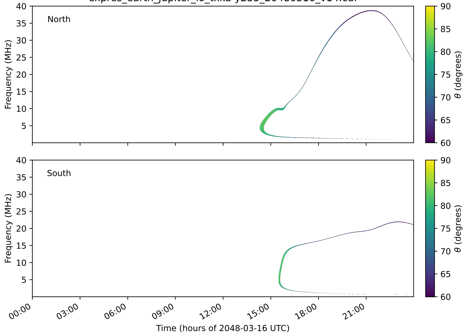
expres_earth_jupiter_io_txka-y235_20480316_v14.cdf
