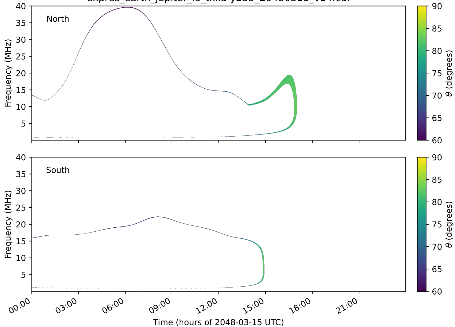
expres_earth_jupiter_io_txka-y235_20480315_v14.cdf
