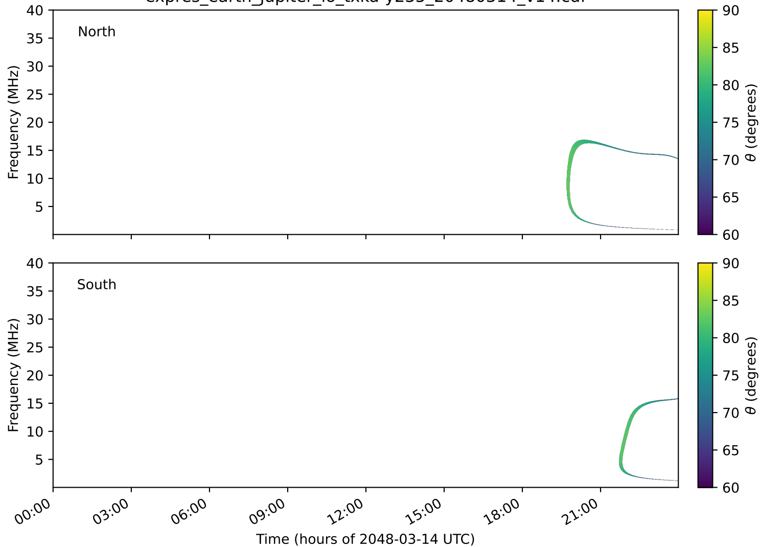
expres_earth_jupiter_io_txka-y235_20480314_v14.cdf
