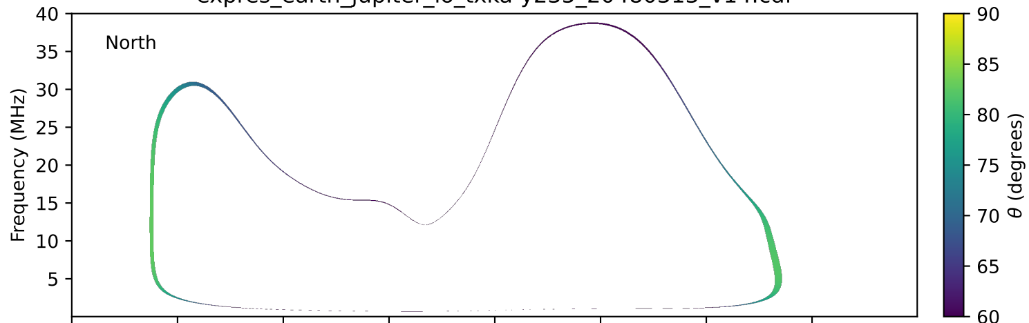
expres_earth_jupiter_io_txka-y235_20480313_v14.cdf
