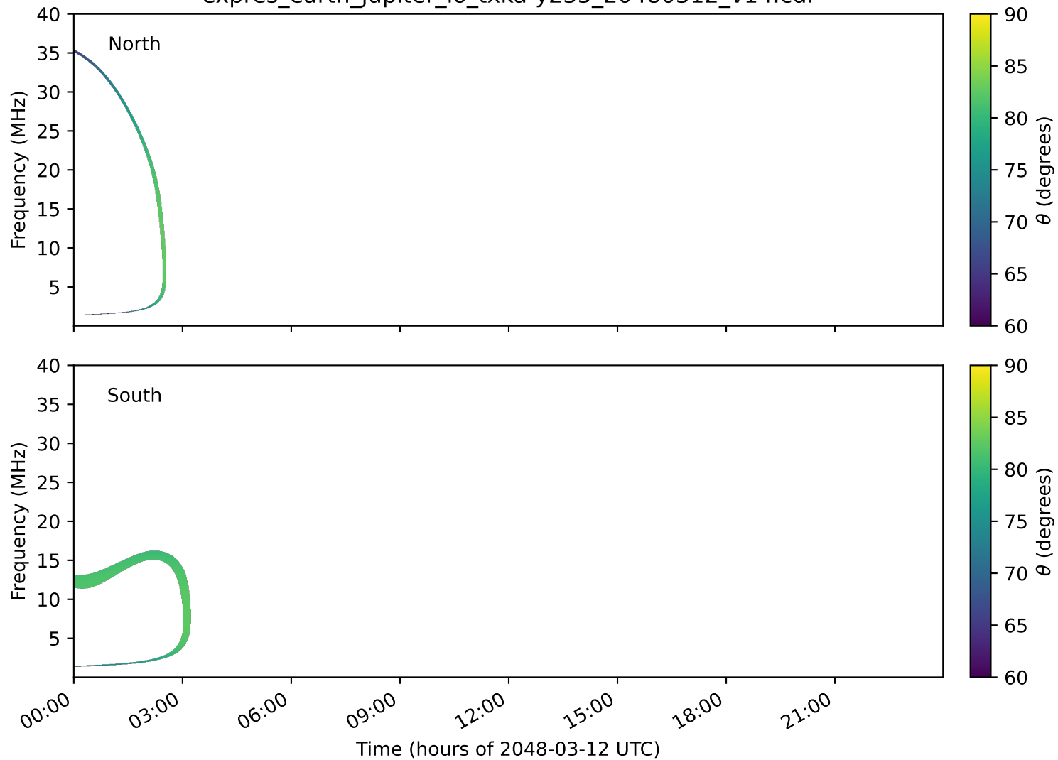
expres_earth_jupiter_io_txka-y235_20480312_v14.cdf
