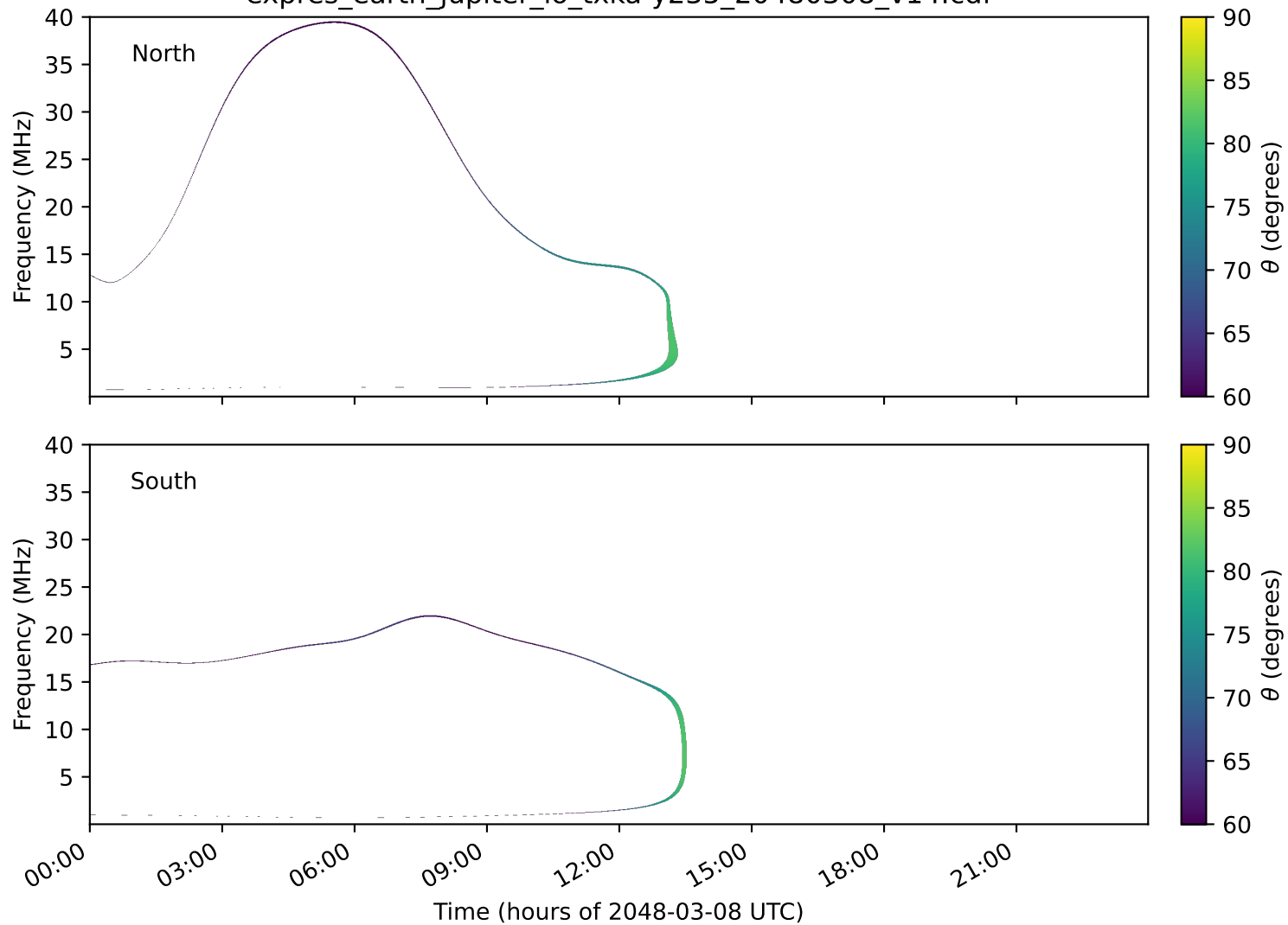
expres_earth_jupiter_io_txka-y235_20480308_v14.cdf
