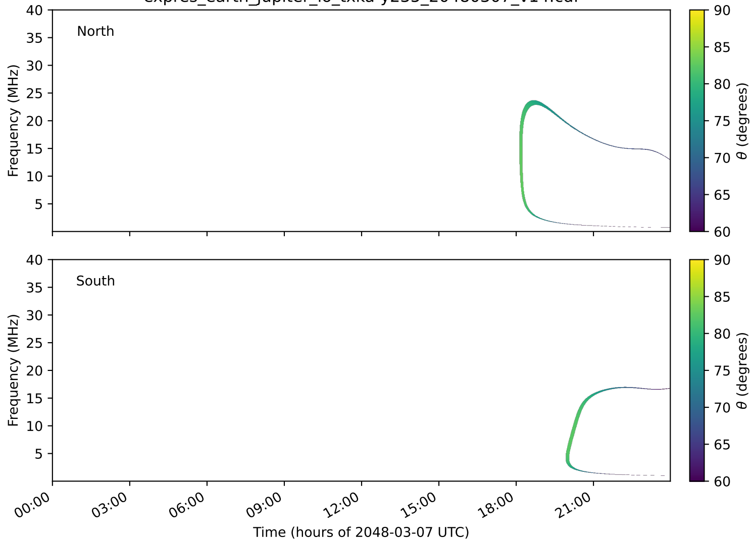
expres_earth_jupiter_io_txka-y235_20480307_v14.cdf
