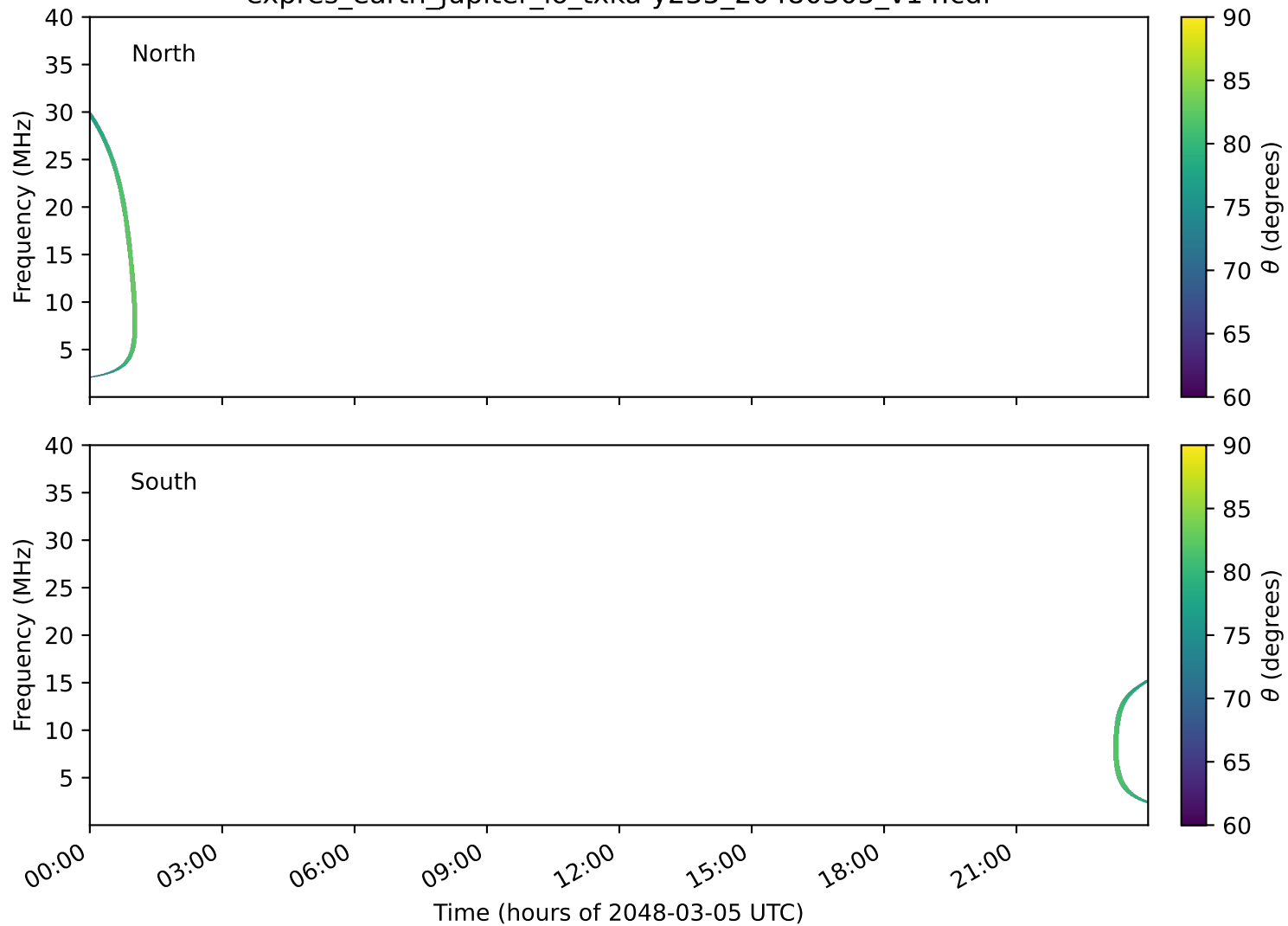
expres_earth_jupiter_io_txka-y235_20480305_v14.cdf
