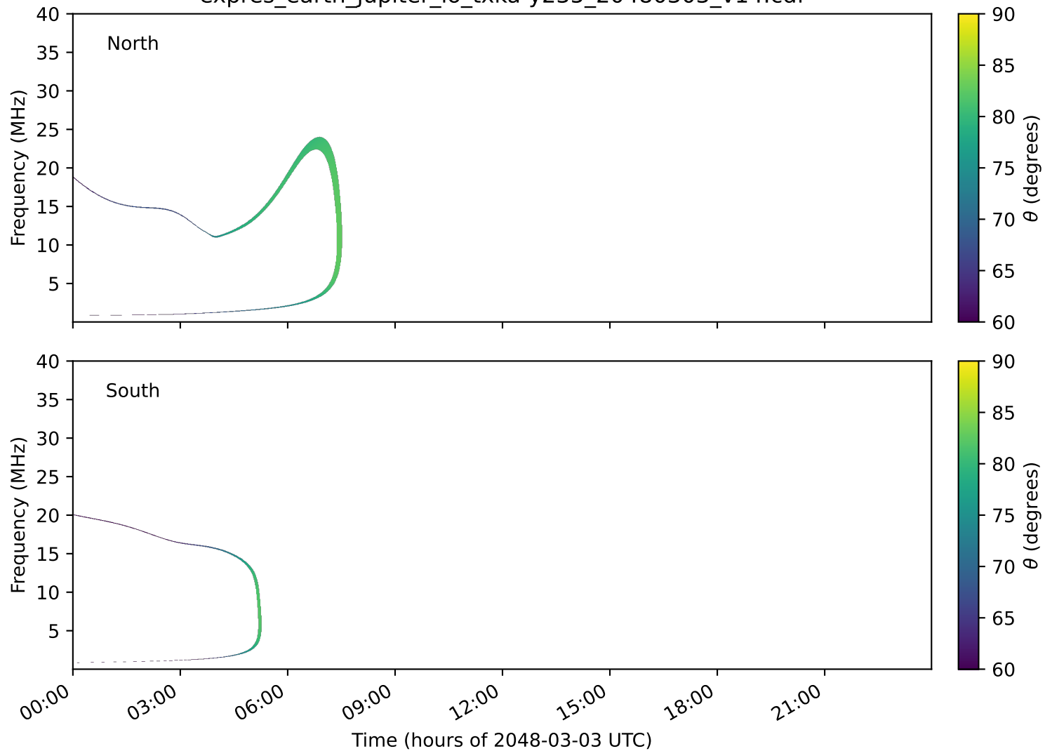
expres_earth_jupiter_io_txka-y235_20480303_v14.cdf
