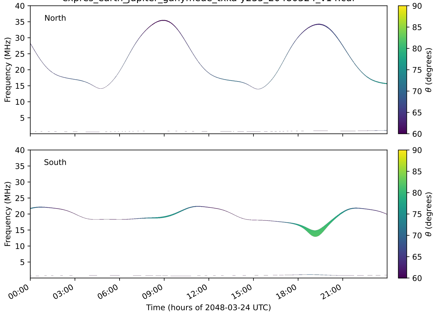
expres_earth_jupiter_ganymede_txka-y235_20480324_v14.cdf
