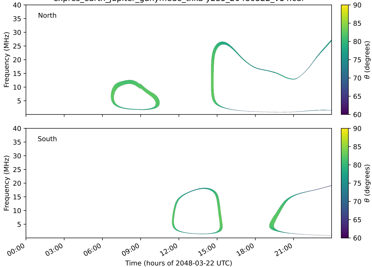
expres_earth_jupiter_ganymede_txka-y235_20480322_v14.cdf
