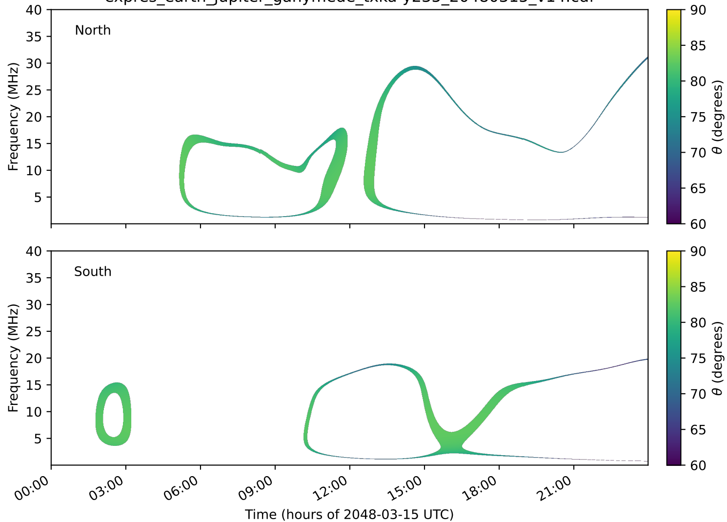
expres_earth_jupiter_ganymede_txka-y235_20480315_v14.cdf
