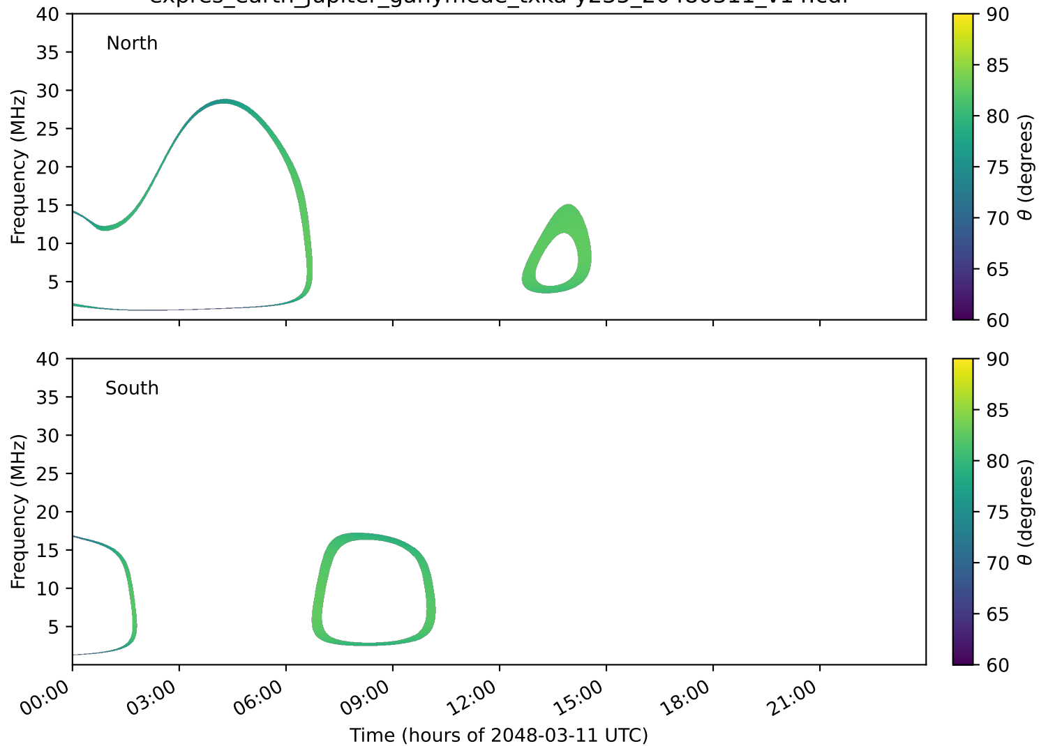
expres_earth_jupiter_ganymede_txka-y235_20480311_v14.cdf
