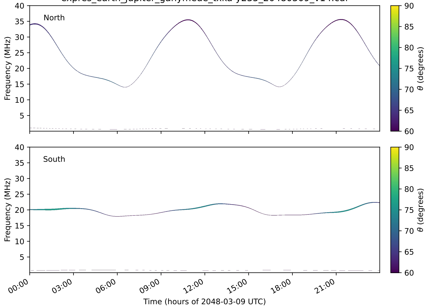
expres_earth_jupiter_ganymede_txka-y235_20480309_v14.cdf
