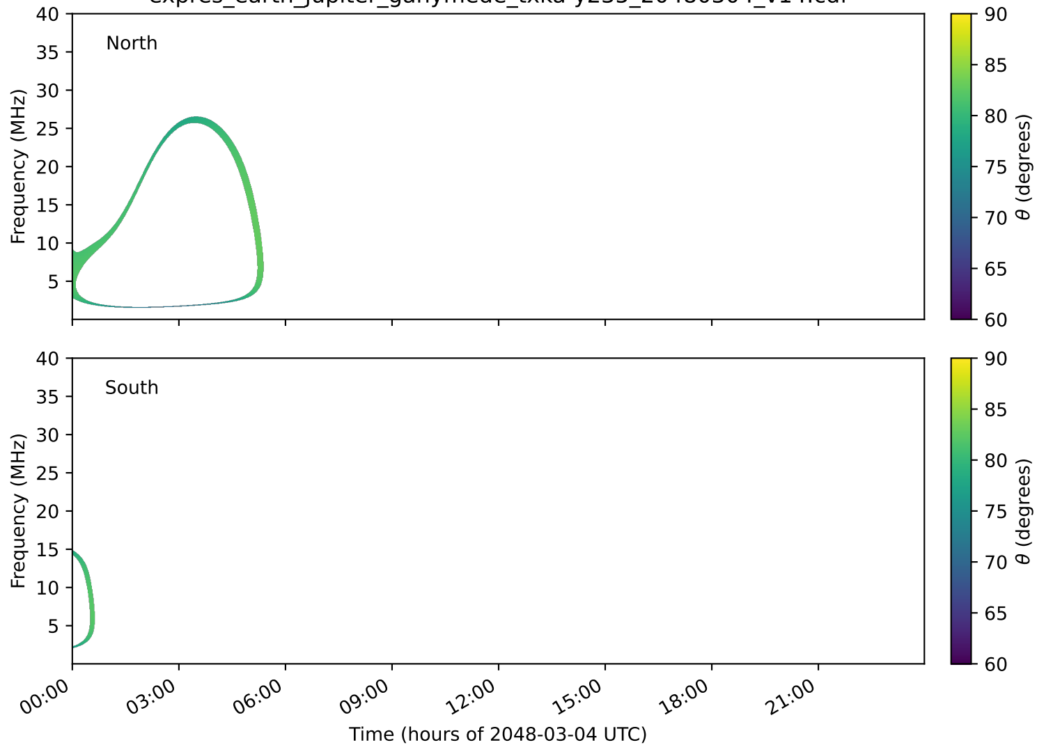
expres_earth_jupiter_ganymede_txka-y235_20480304_v14.cdf
