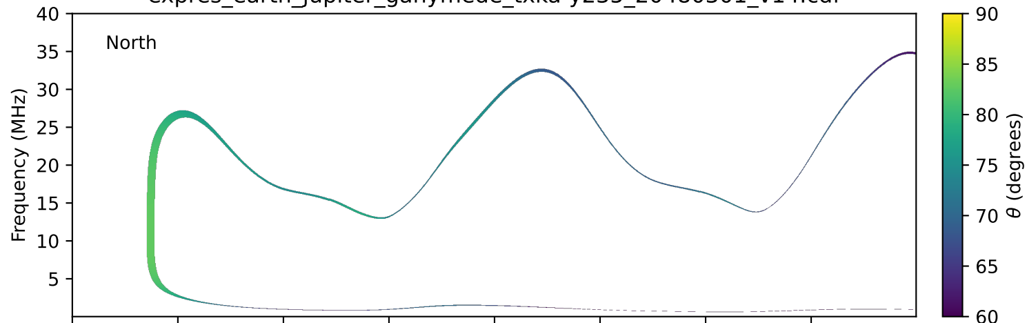
expres_earth_jupiter_ganymede_txka-y235_20480301_v14.cdf
