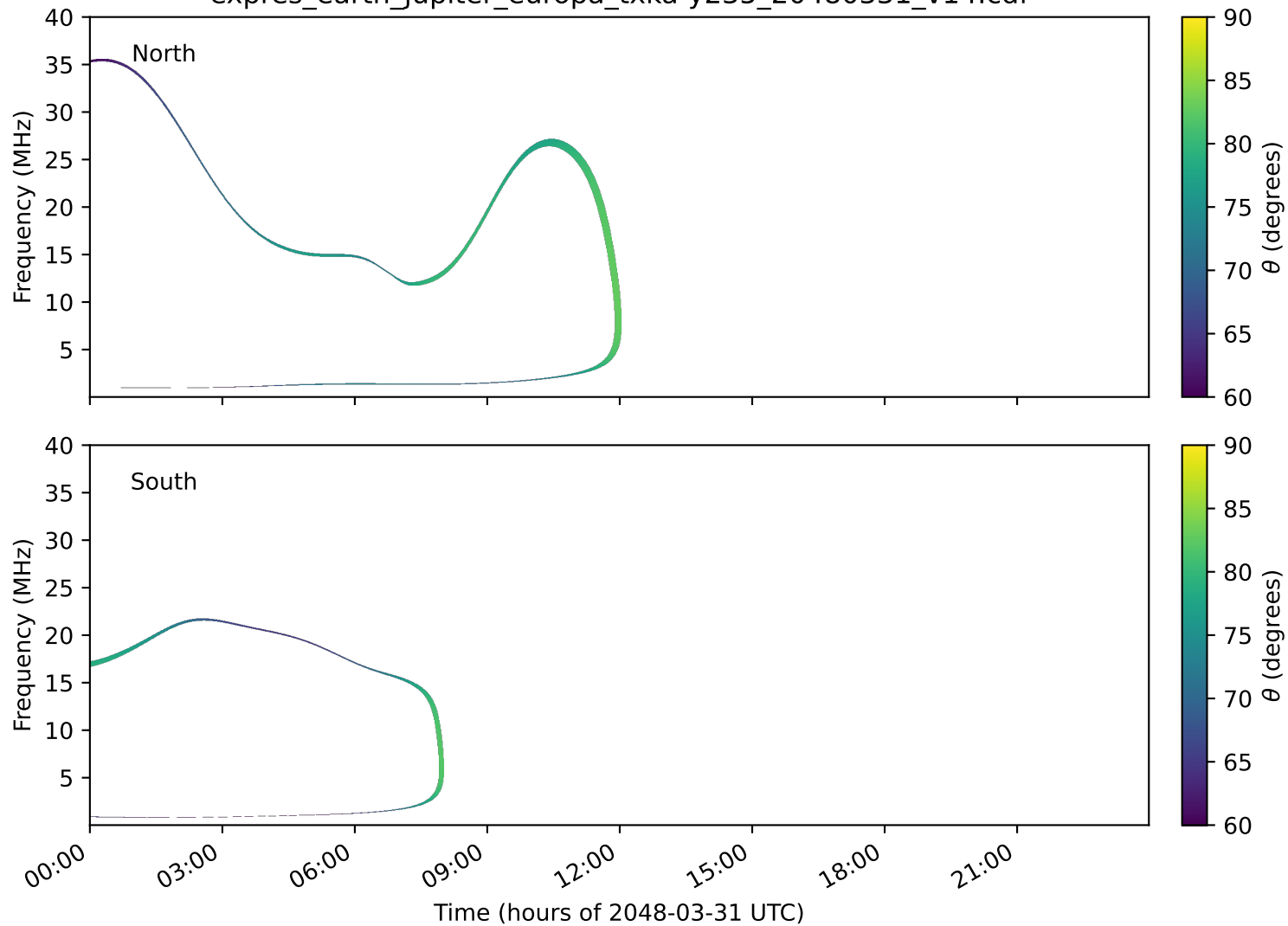
expres_earth_jupiter_europa_txka-y235_20480331_v14.cdf
