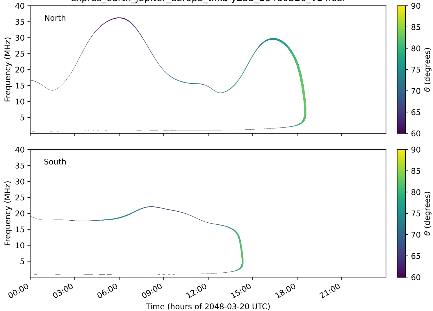
expres_earth_jupiter_europa_txka-y235_20480320_v14.cdf
