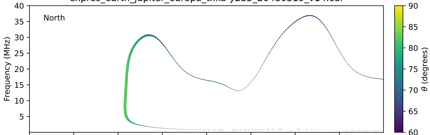
expres_earth_jupiter_europa_txka-y235_20480319_v14.cdf
