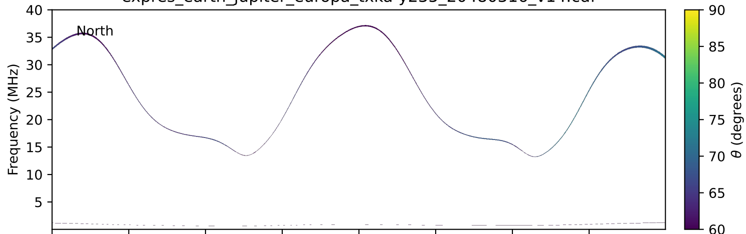
expres_earth_jupiter_europa_txka-y235_20480316_v14.cdf
