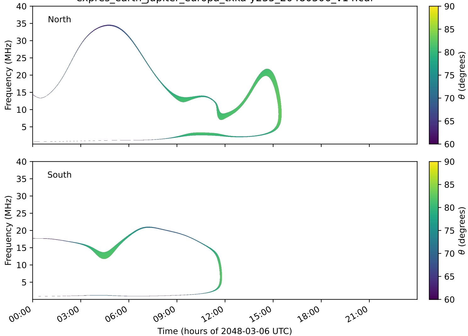
expres_earth_jupiter_europa_txka-y235_20480306_v14.cdf
