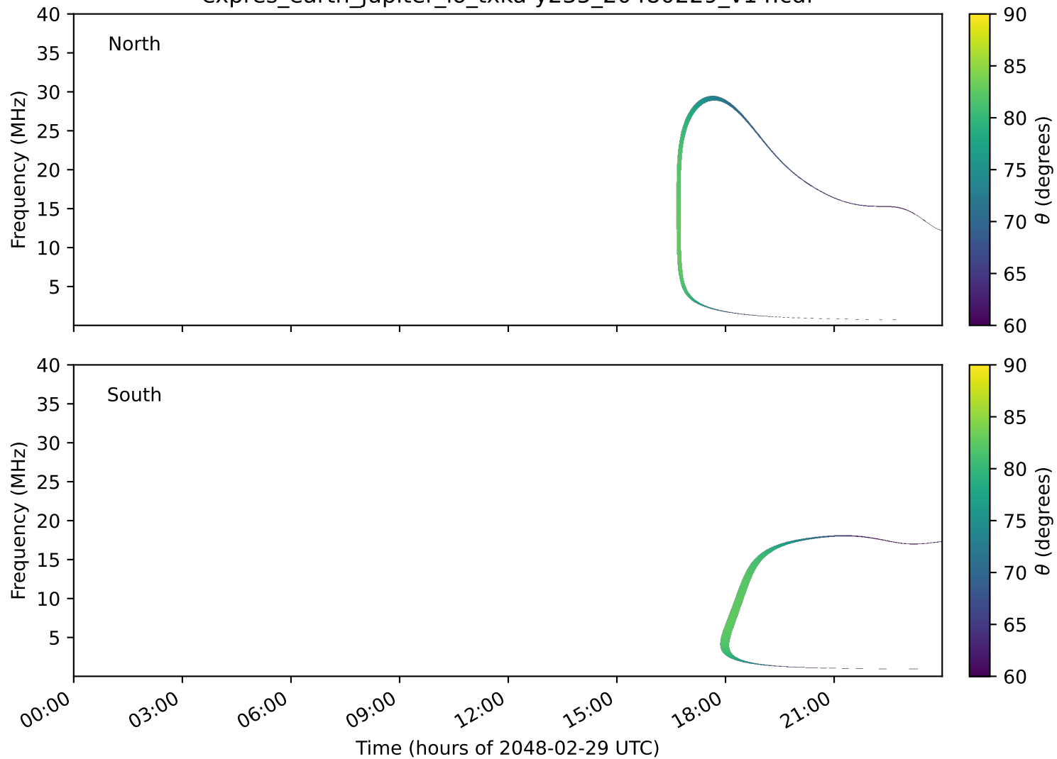
expres_earth_jupiter_io_txka-y235_20480229_v14.cdf
