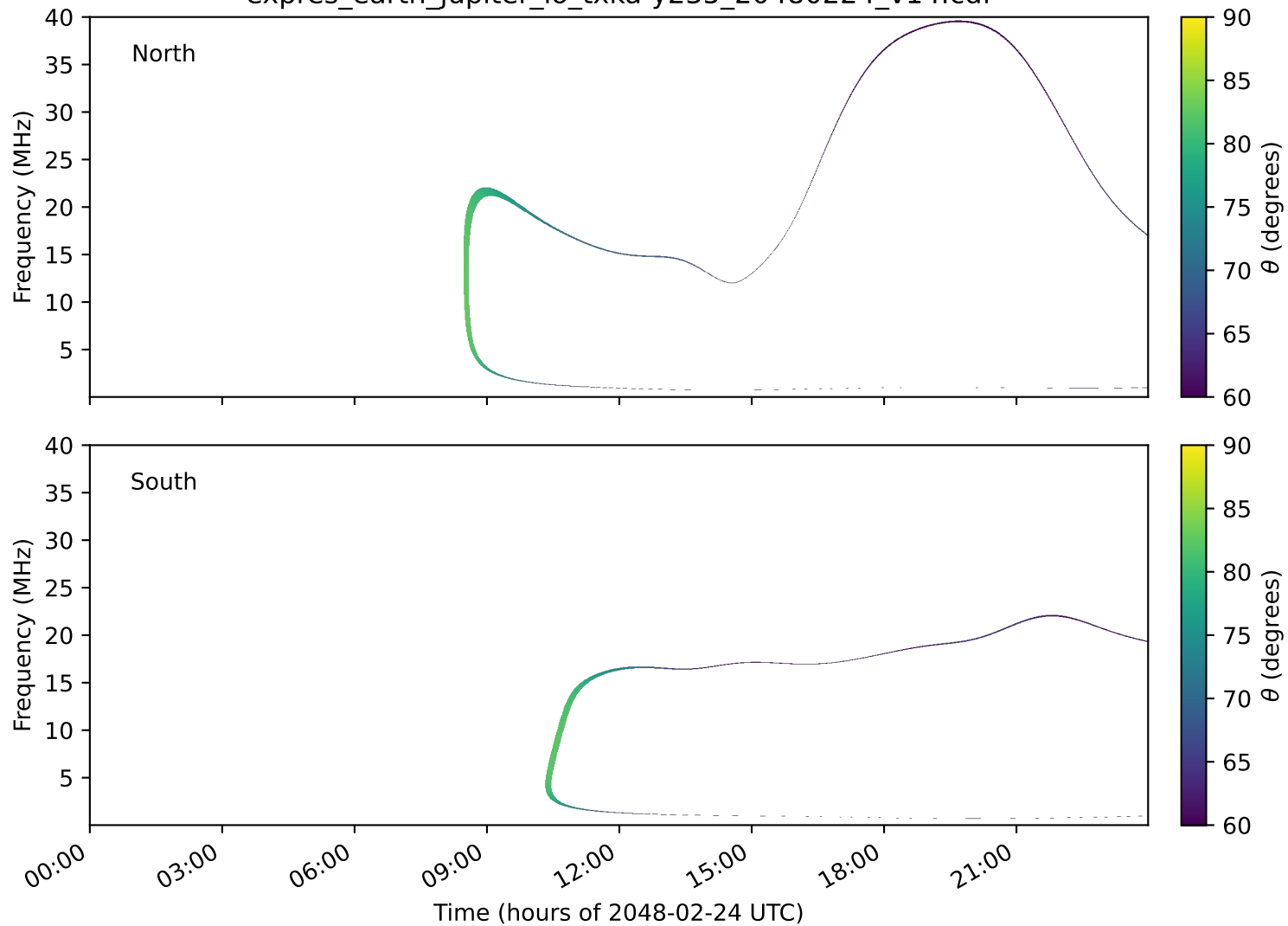
expres_earth_jupiter_io_txka-y235_20480224_v14.cdf
