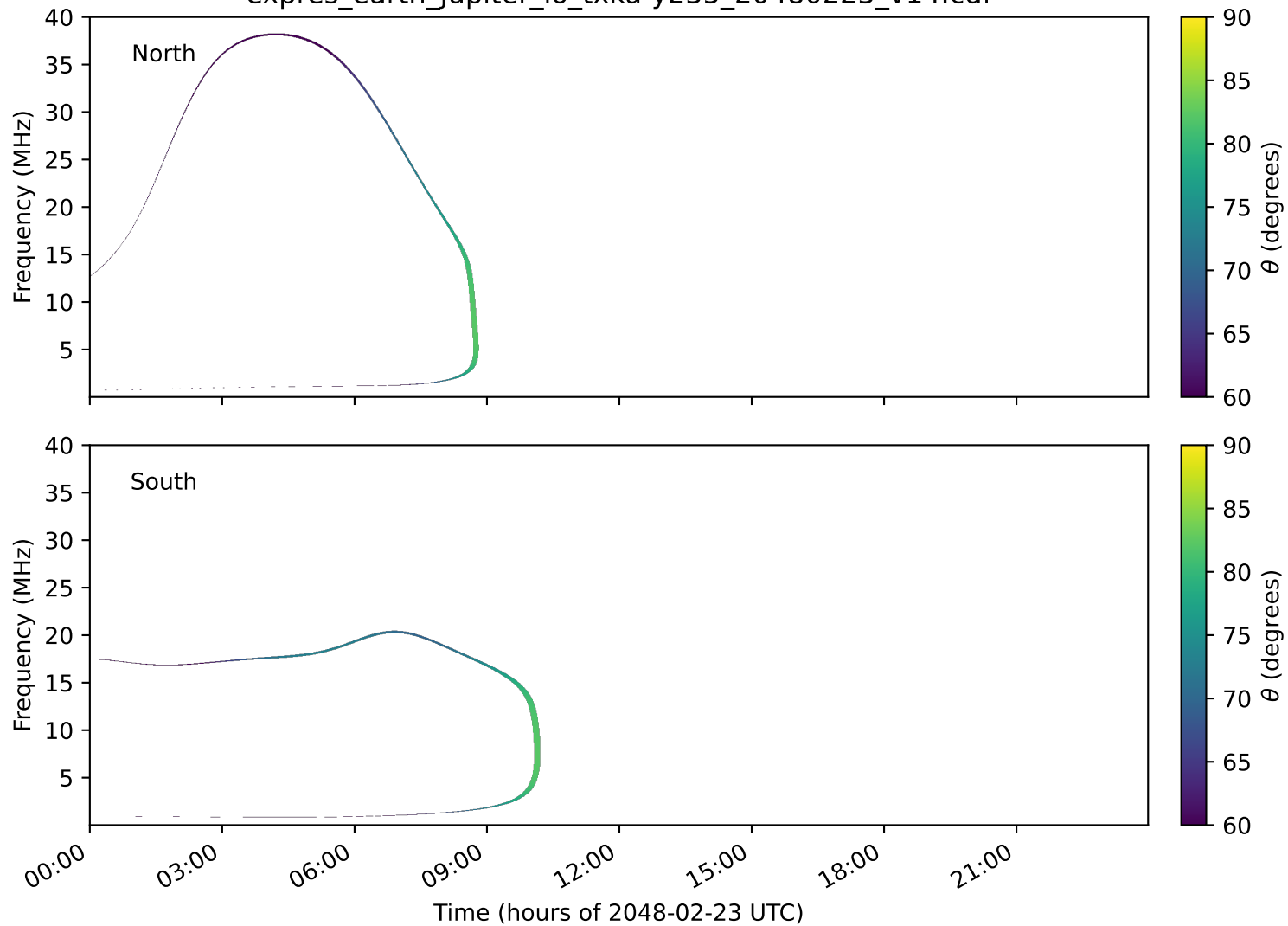
expres_earth_jupiter_io_txka-y235_20480223_v14.cdf
