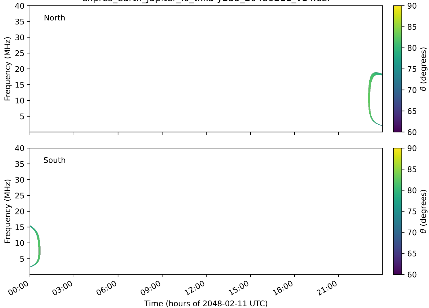
expres_earth_jupiter_io_txka-y235_20480211_v14.cdf
