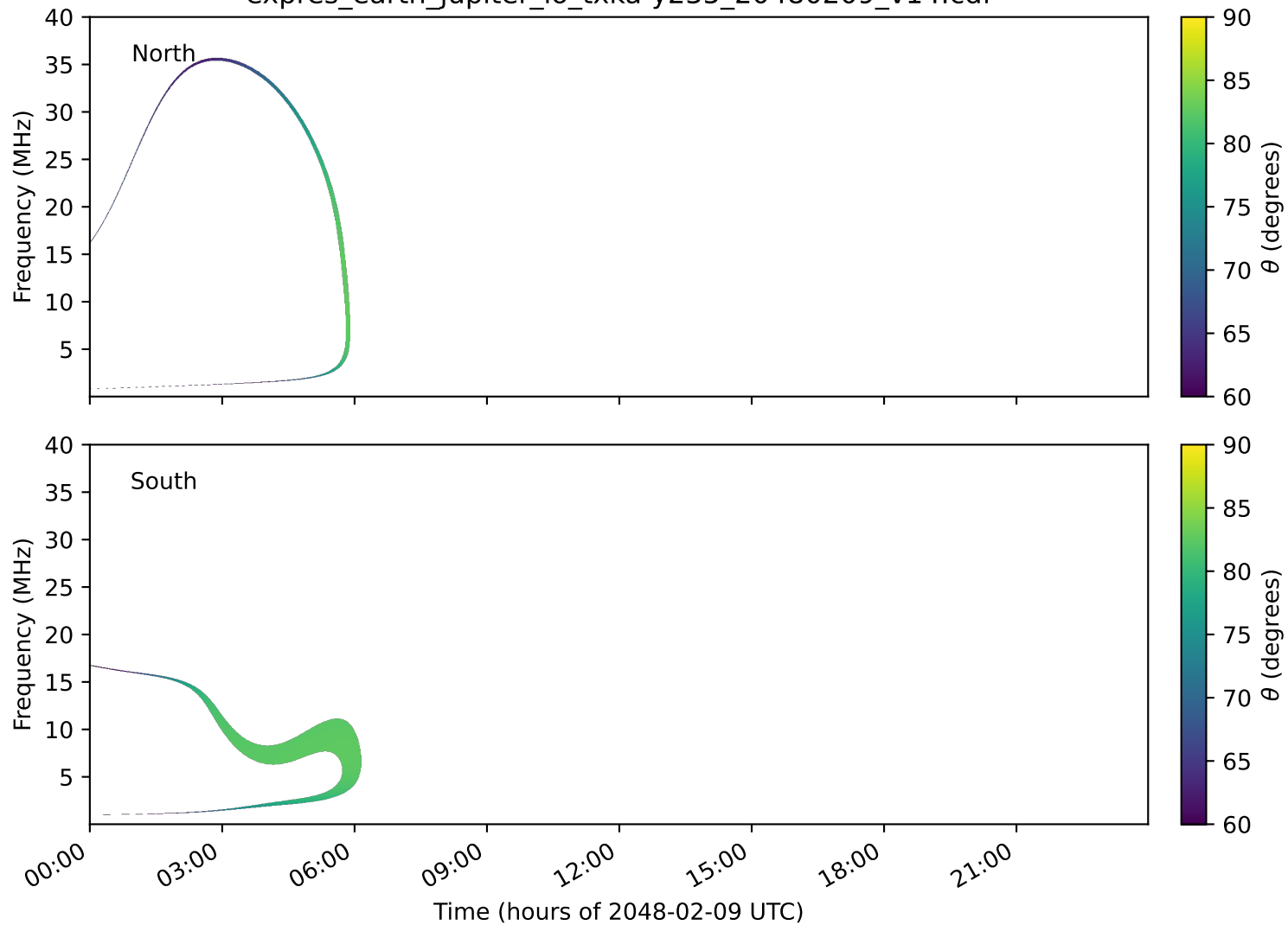
expres_earth_jupiter_io_txka-y235_20480209_v14.cdf
