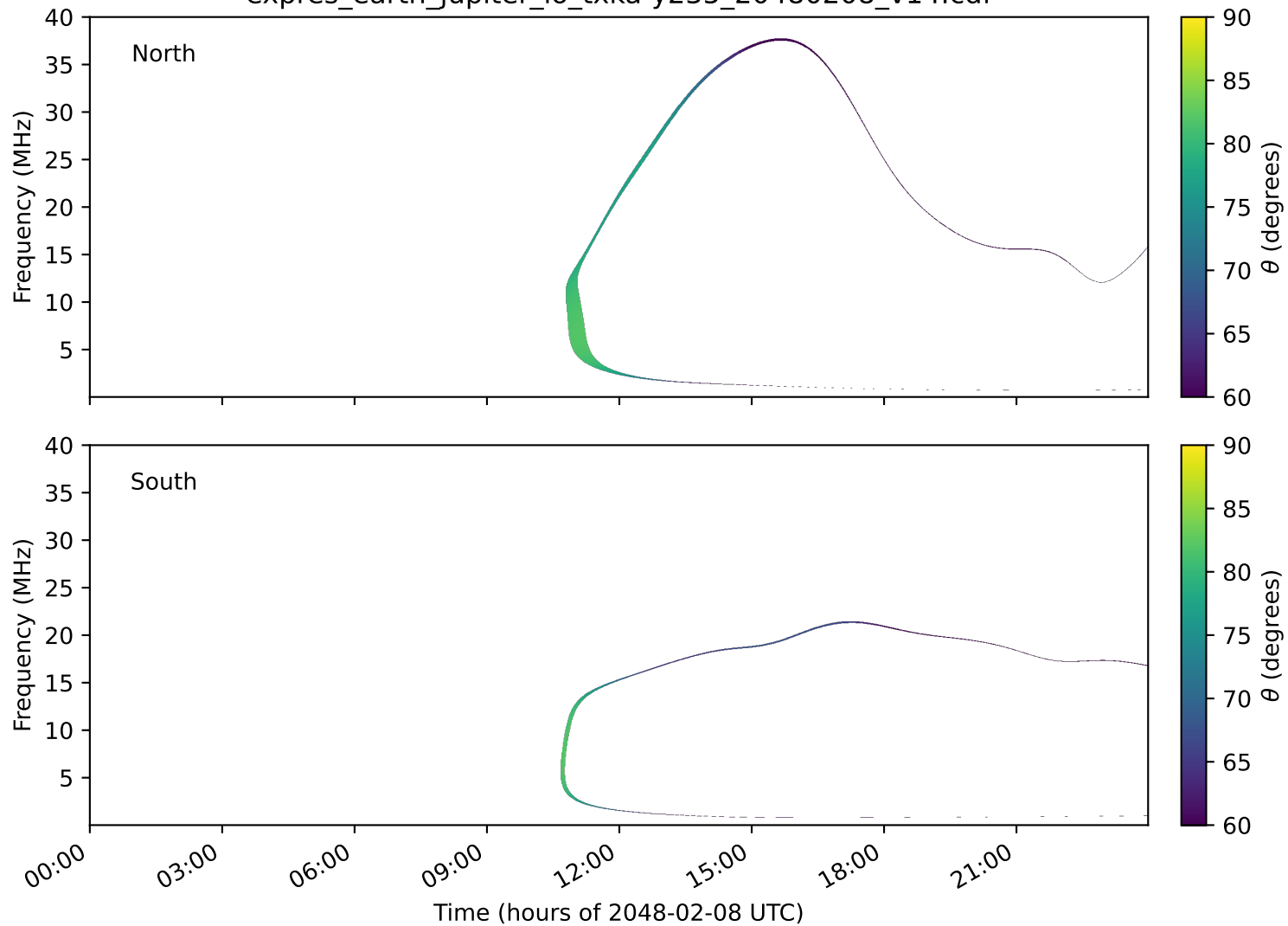
expres_earth_jupiter_io_txka-y235_20480208_v14.cdf
