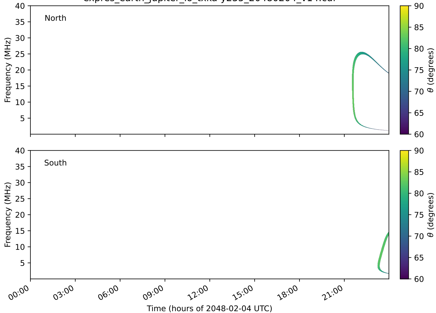
expres_earth_jupiter_io_txka-y235_20480204_v14.cdf
