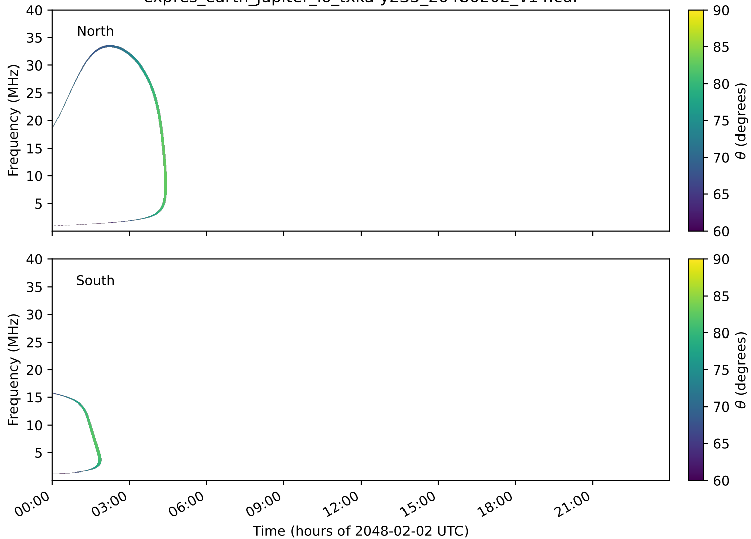
expres_earth_jupiter_io_txka-y235_20480202_v14.cdf
