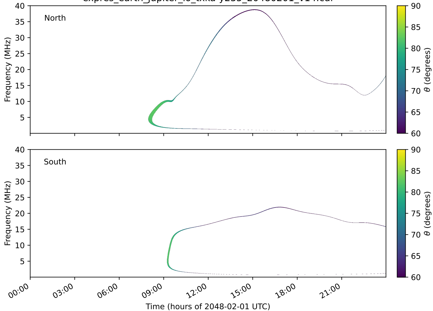
expres_earth_jupiter_io_txka-y235_20480201_v14.cdf
